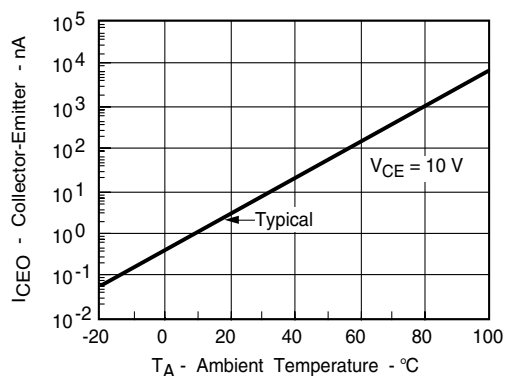
Fig. 9 Collector-Emmitter Leakage vs. Temperature
