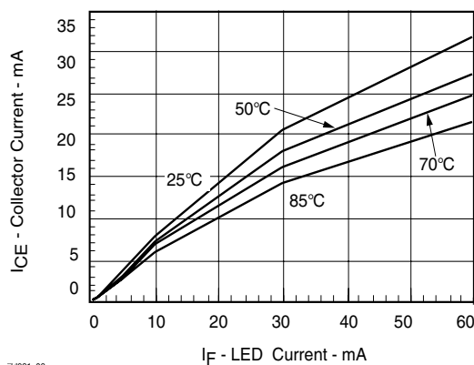
Fig. 8 Collector-Emmitter Current vs. Temperature and LED Current
