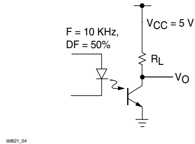
Fig. 4 Saturated Switching Timing
