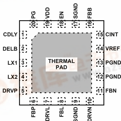
EL7585 (20-PIN QFN) TOP VIEW
