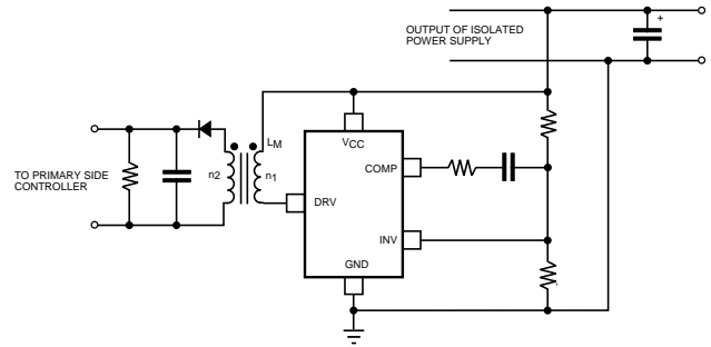
FIGURE 5: ISOLATING THE ERROR SIGNAL WITH A PULSE TRANSFORMER
