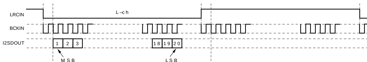
Figure 75. Audio Data Input/Output Format
