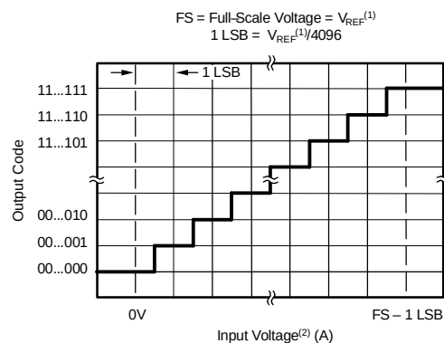
Figure 48. Ideal Input Voltages and Output Codes.
