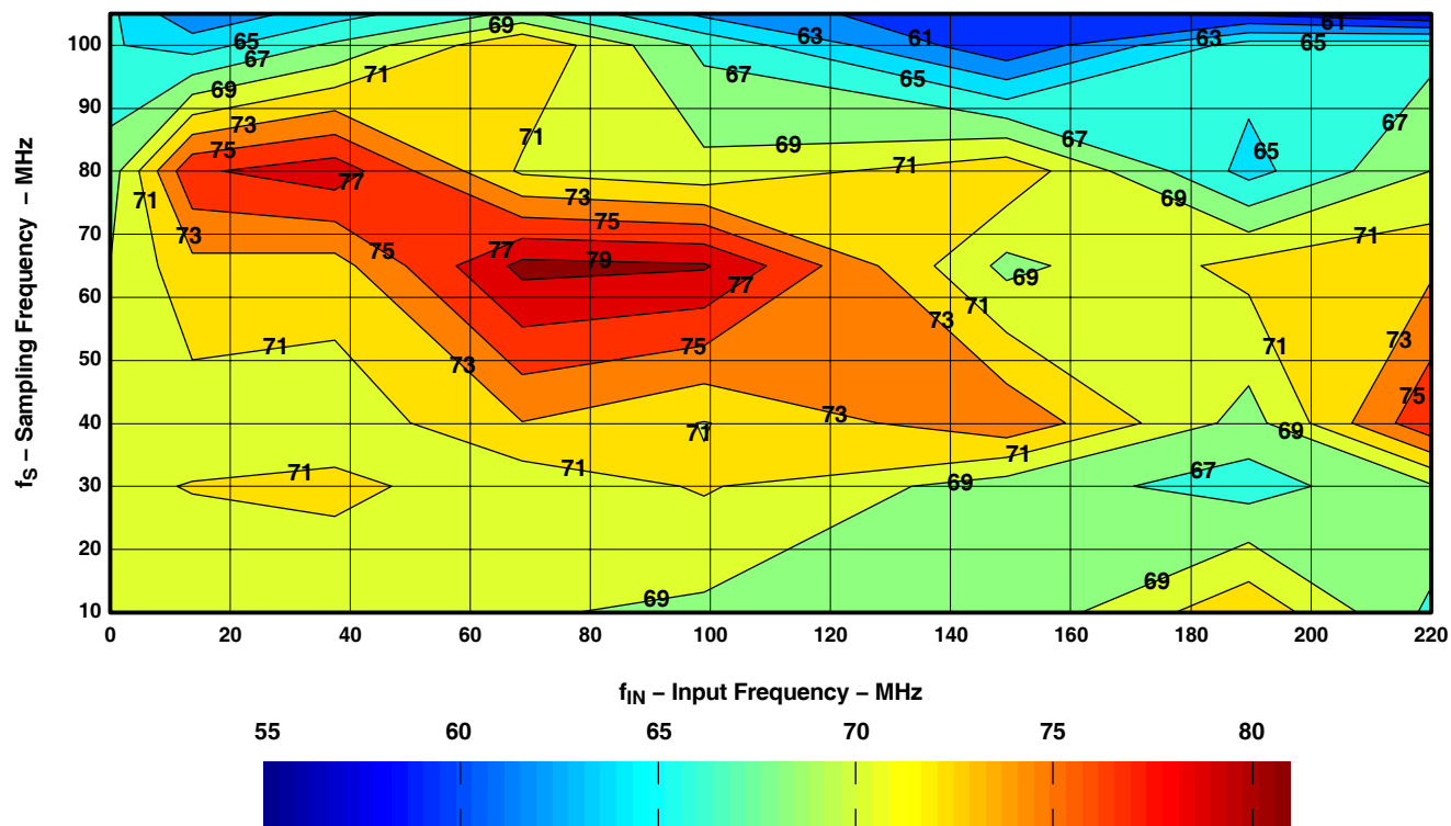
Figure 15. SFDR – dBc
