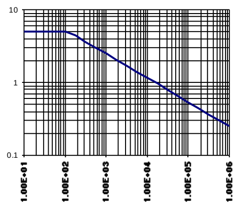
Figure 10 - Max. I_{out} (A) Vs Load Inductance (μH)
