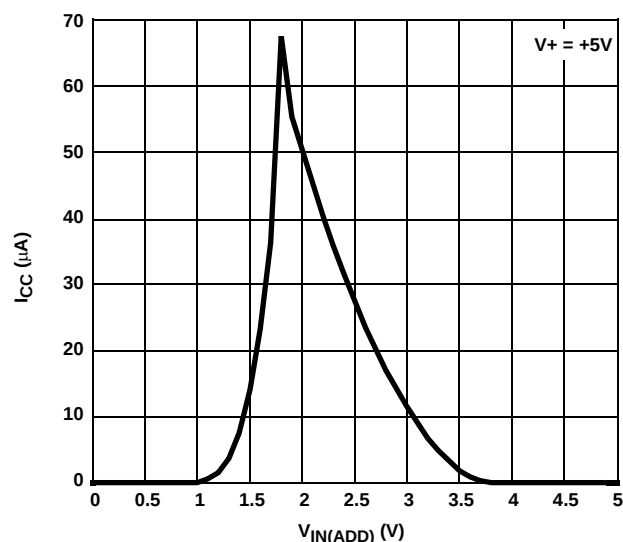
FIGURE 11. SUPPLY CURRENT vs DIGITAL ADDRESS INPUT VOLTAGE
