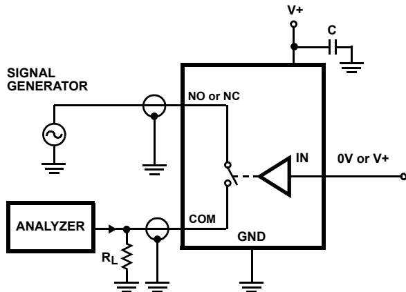
FIGURE 3. BREAK-BEFORE-MAKE TIME
