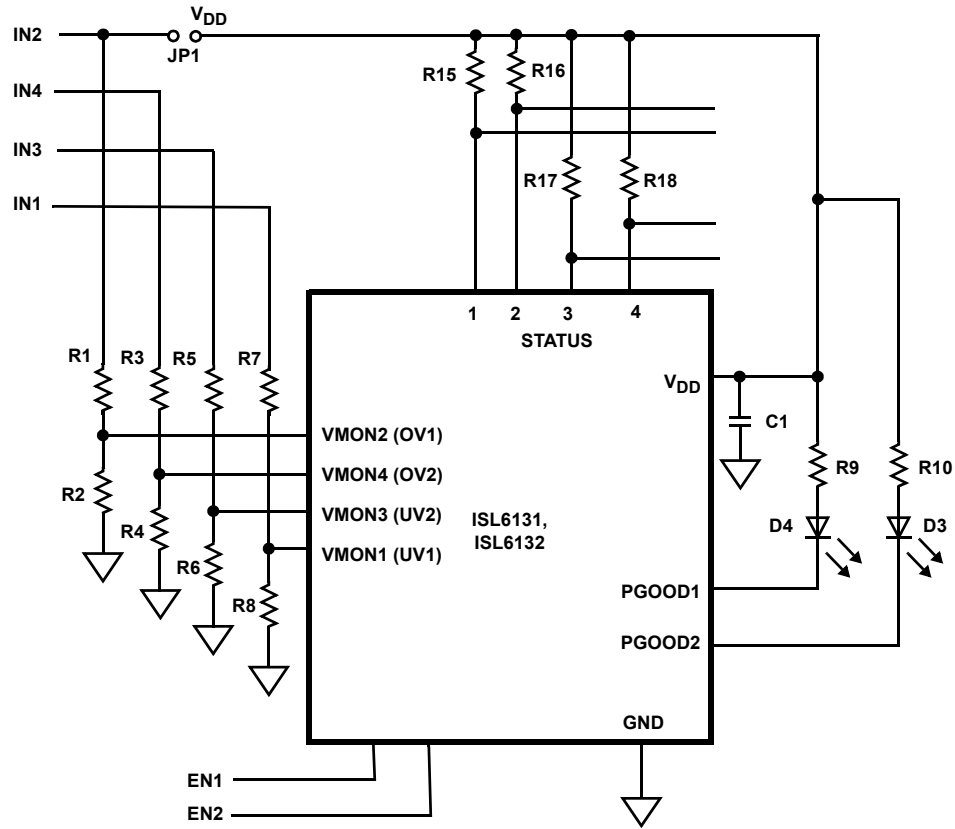
FIGURE 26. ISL6131SUPEREVAL2 CHANNEL 1 SCHEMATIC
