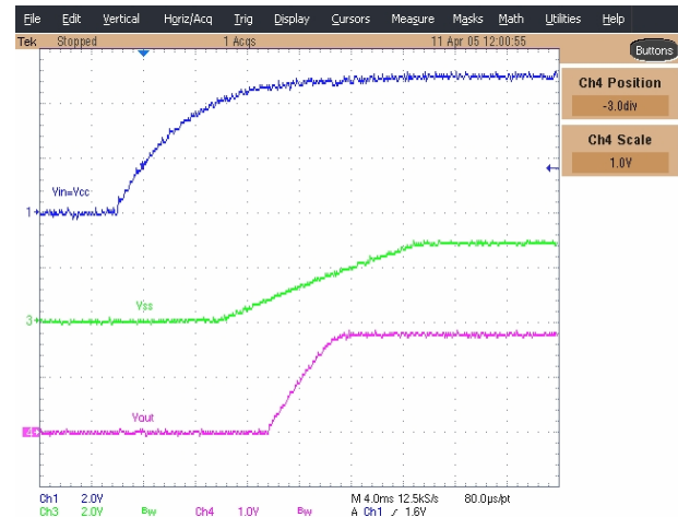
Figure 5 - Start up waveforms Ch1: V_{in}=V_{cc} , Ch2: V_c , Ch3: V_{ss} , Ch4: V_{out}
