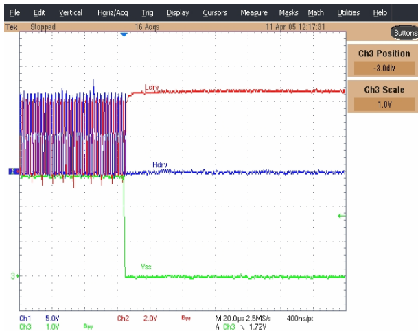
Figure 8 - Shutdown by shorting the SS pin Ch1: Hdrv, Ch2:Ldrv,, Ch3:SS I_{Load}=5A
