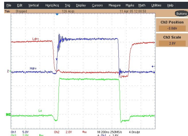
Figure 7 - Gates waveforms Ch1: Hdrv, Ch2:Ldrv,, Ch3:Inductor Point I_{Load}=5A
