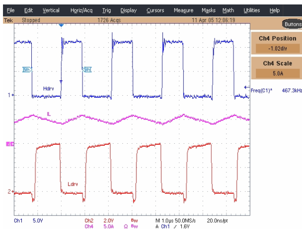
Figure 6 - Gates waveforms Ch1: Hdrv, Ch2:Ldrv,, Ch4:Inductor Current I_{Load}=5A
