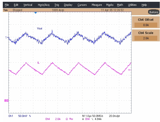
Figure 9 - Output Voltage Ripple Ch1: Vout, Ch4: Inductor Current I_{Load}=5A
