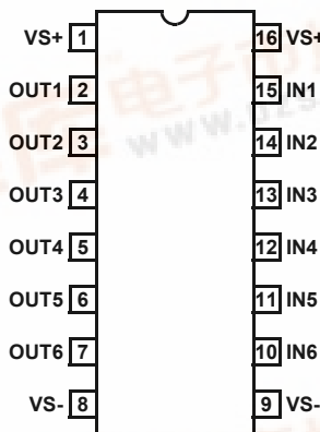
EL5623 (16-PIN TSSOP) TOP VIEW
