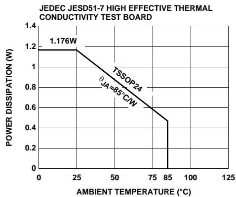
FIGURE 8. PACKAGE POWER DISSIPATION vs AMBIENT TEMPERATURE
