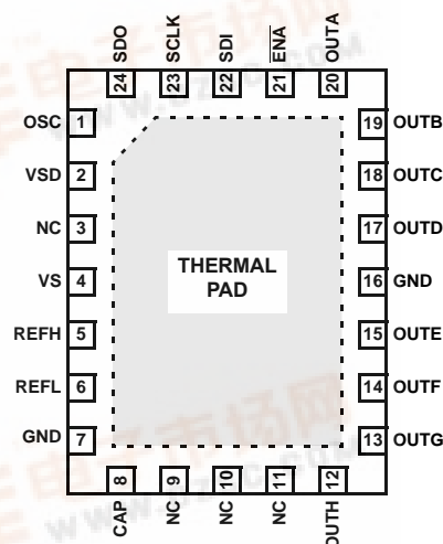
EL5825 (24-PIN QFN) TOP VIEW
