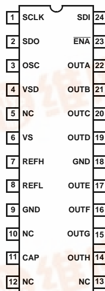
EL5825 (24-PIN TSSOP) TOP VIEW
