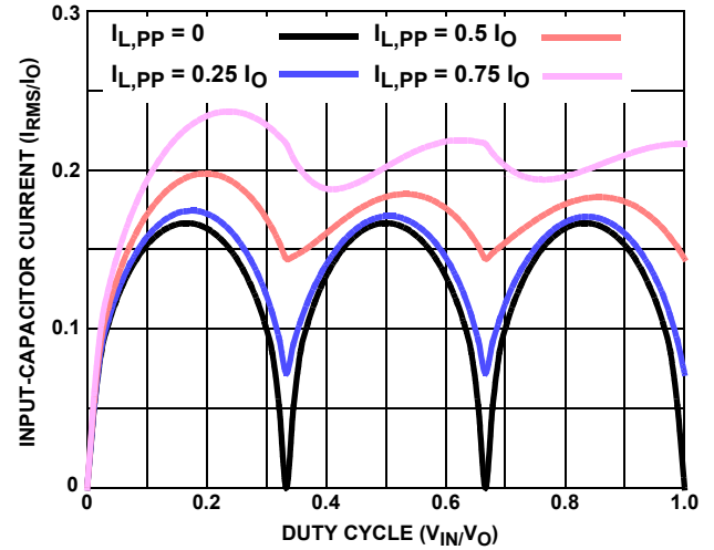
FIGURE 24. NORMALIZED INPUT-CAPACITOR RMS CURRENT FOR 3-PHASE CONVERTER
