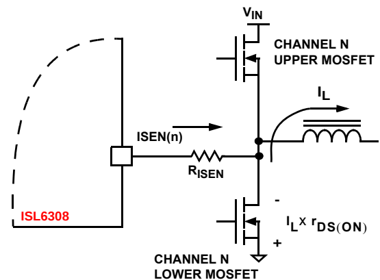
FIGURE 17. ISL6308 INTERNAL AND EXTERNAL CURRENT-SENSING CIRCUITRY
