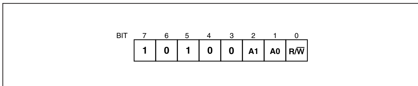
Figure 5. Slave Address
