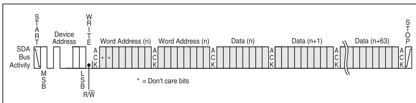
Figure 7. Page Write
