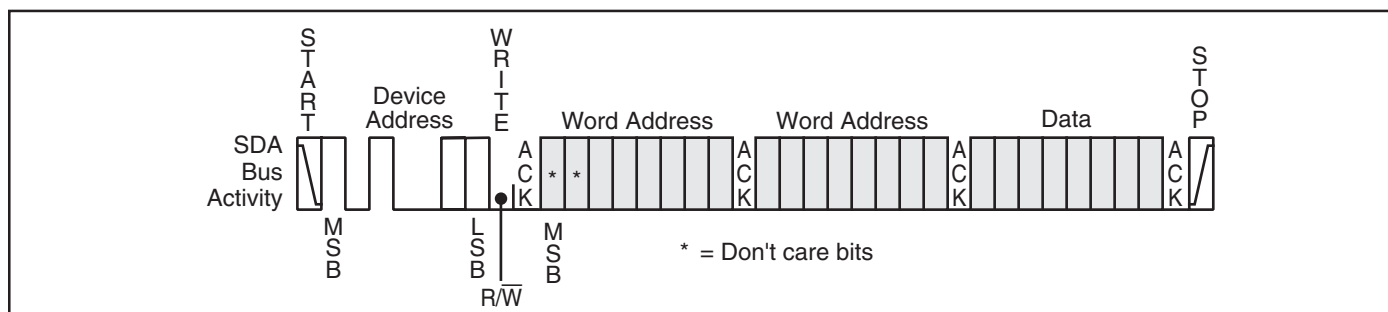
Figure 6. Byte Write
