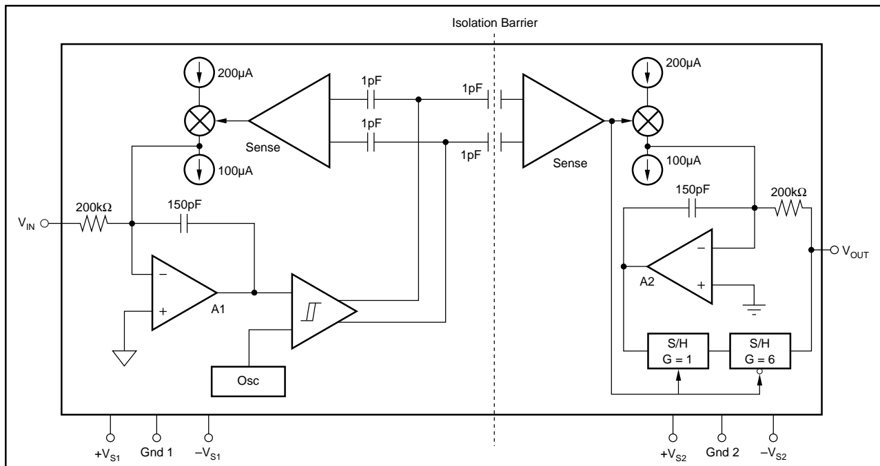
FIGURE 1. Block Diagram.
