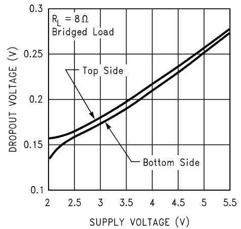
Dropout Voltage
