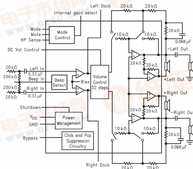
FIGURE 1. LM4838 Block Diagram
