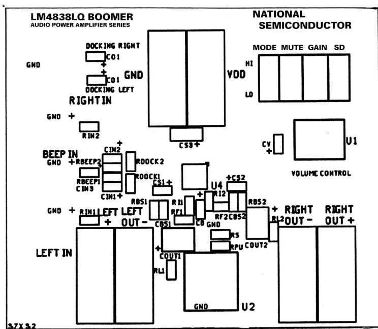
FIGURE 5. Recommended LQ PC Board Layout: Component-Side Silkscreen
