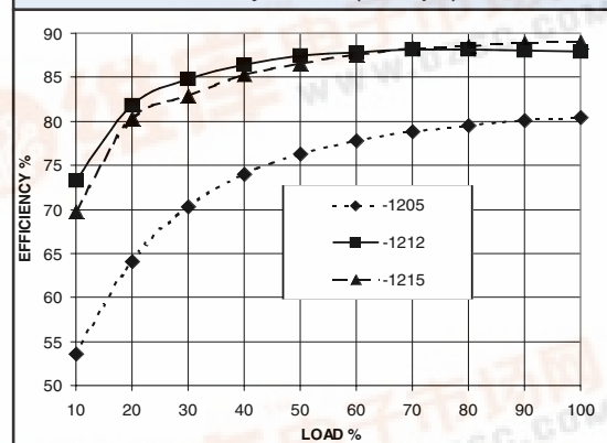
Efficiency vs. Load (12V Input)
