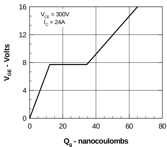
Fig.9. Gate Charge
