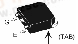
TO-268
