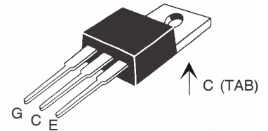
TO-220AB (IXSP)
