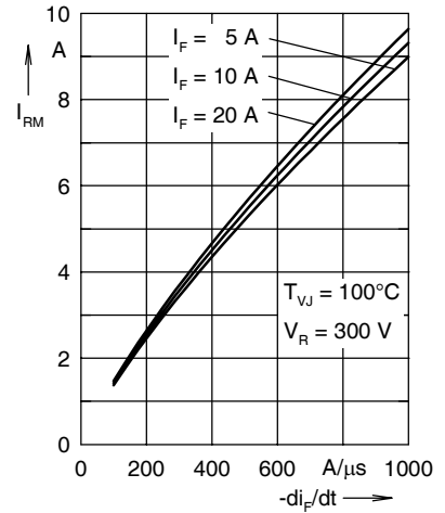
Fig. 20. Peak reverse current I_{RM} versus -di_F/dt
