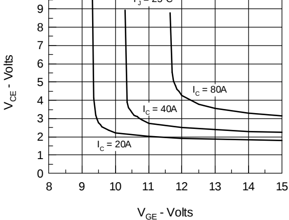
Fig. 3 Collector-Emitter Voltage vs. Gate-Emitter Voltage
