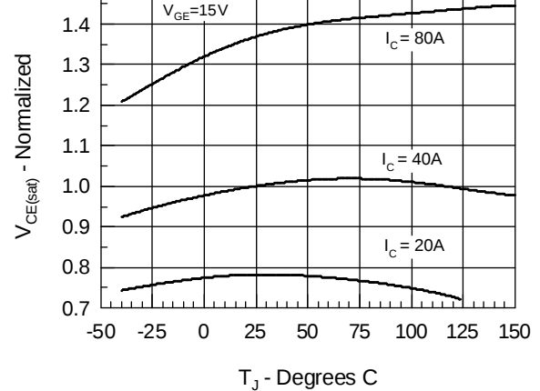
Fig. 4 Temperature Dependence of Output Saturation Voltage
