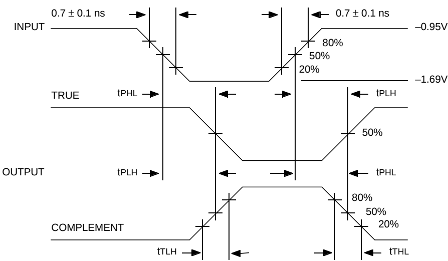
Propagation Delay and Transition Times
