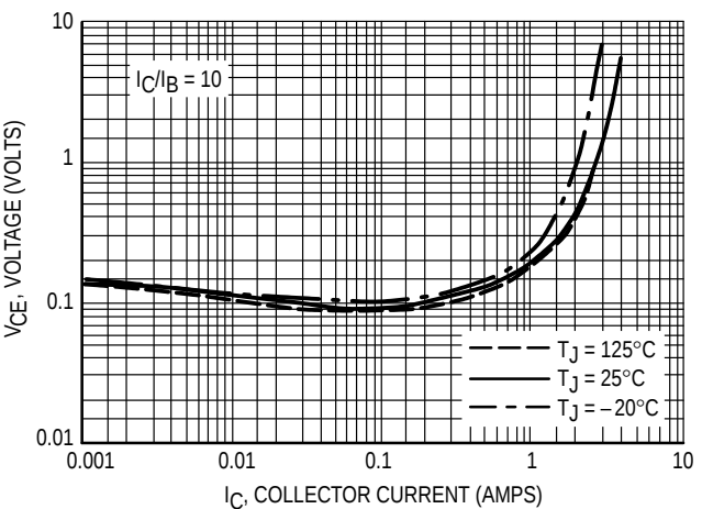
Figure 5B. Collector-Emmitter Saturation Voltage
