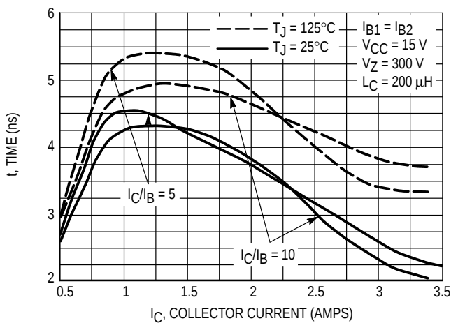
Figure 10. Inductive Storage Time, t_{sj}
