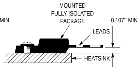
Figure 26. Screw Mounting Position for Isolation Test Number 3
