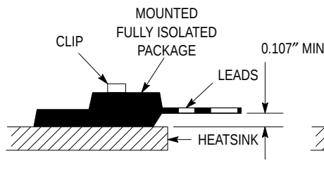
Figure 25. Clip Mounting Position for Isolation Test Number 2
