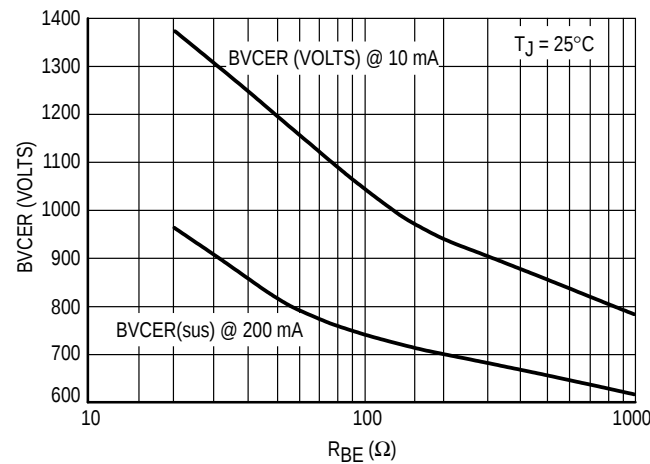
Figure 16. BVCER = f(R_{BE})
