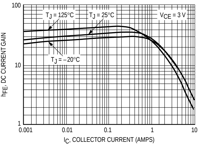
Figure 2. DC Current Gain @ 3 Volts
