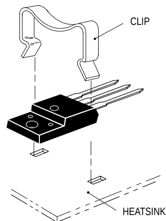
Figure 27b. Clip-Mounted
