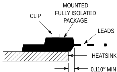
Figure 24. Clip Mounting Position for Isolation Test Number 1
