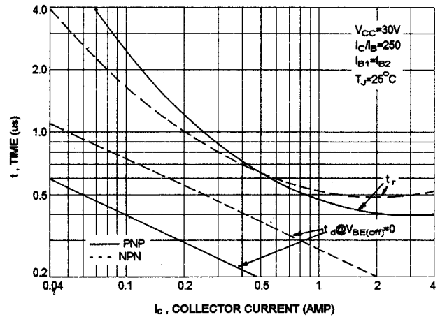
FIG-3 TURN-ON TIME
