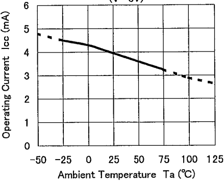
Operating Current vs. Temperature ( V^+=5\text{V} )
