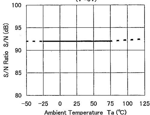
S/N Ratio vs. Temperature ( V^+=5\text{V} )
