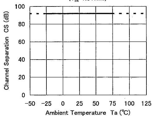
Channel Separation vs. Temperature ( V_{IN}=1.5\text{Vrms} )
