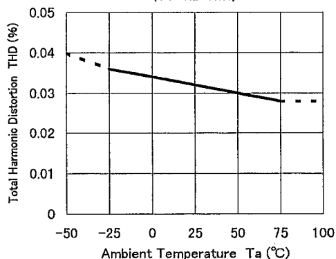
Total Harmonic Distortion vs. Temperature ( V_o=0.2\text{Vrms} )
