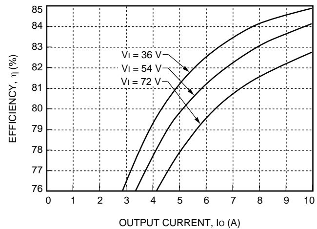
Figure 9. Typical JW050A Converter Efficiency vs. Output Current at Room Temperature
