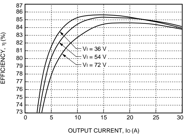
Figure 12. Typical JW150A Converter Efficiency vs. Output Current at Room Temperature
