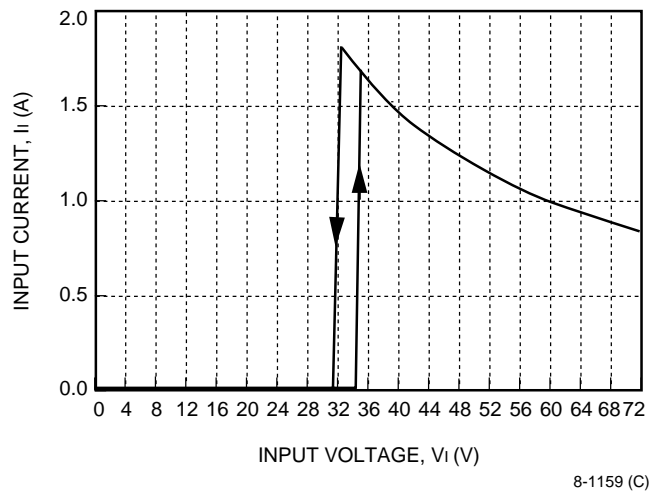
Figure 1. Typical JW050A Input Characteristics at Room Temperature
