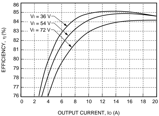
Figure 11. Typical JW100A Converter Efficiency vs. Output Current at Room Temperature
