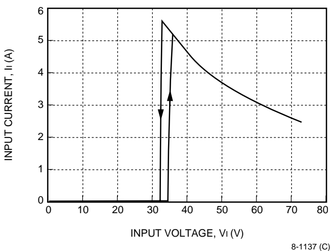
Figure 4. Typical JW150A Input Characteristics at Room Temperature
