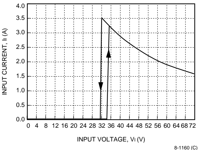
Figure 3. Typical JW100A Input Characteristics at Room Temperature
