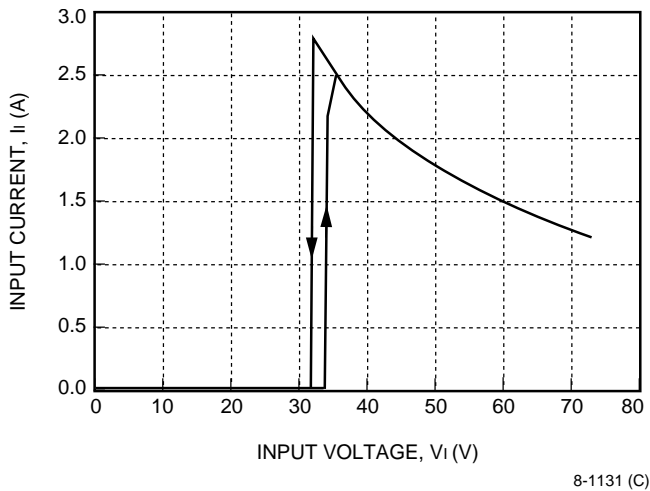
Figure 2. Typical JW075A Input Characteristics at Room Temperature
