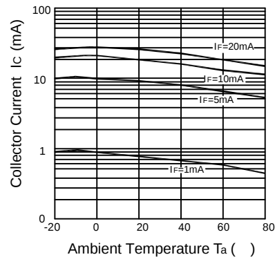
Collector Current vs. Ambient Temperature
