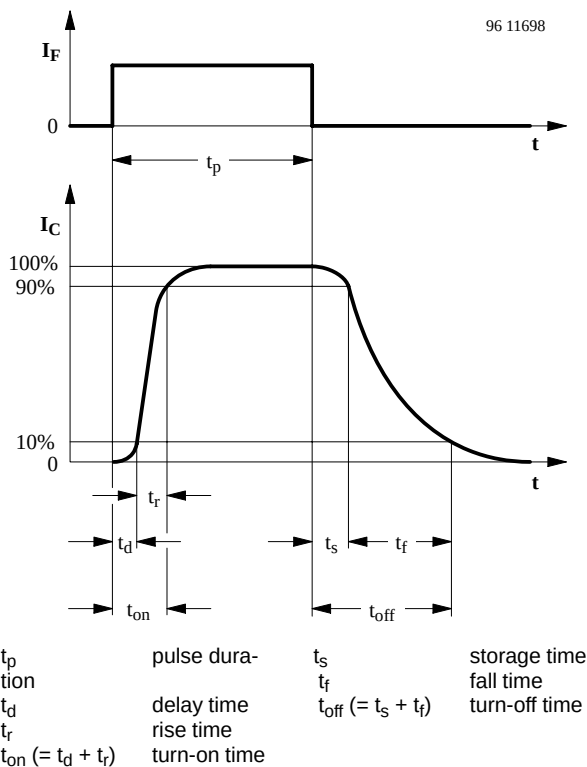
Figure 3. Switching times
