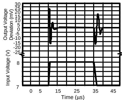
Figure 10.Line Transient Response
