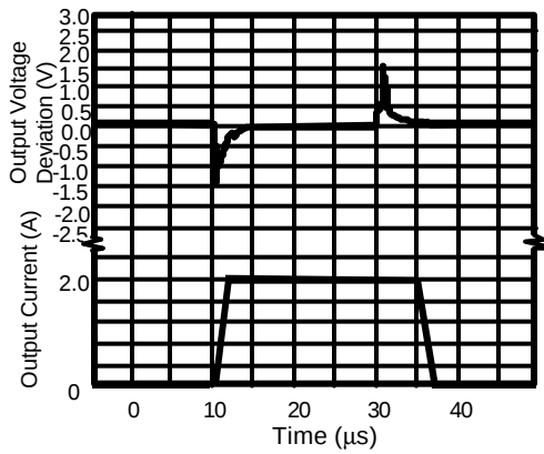
Figure 11.Load Transient Response
