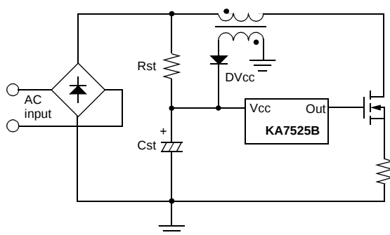
Figure 1.1 Start-up Circuit
