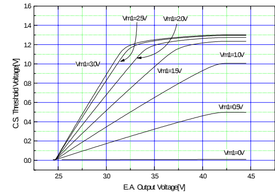
Figure 1. E.A. Output Voltage vs C.S. Threshold
