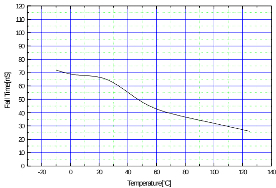
Figure 17. Fall Time vs Temperature
