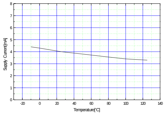
Figure 18. Supply Current vs Temperature
