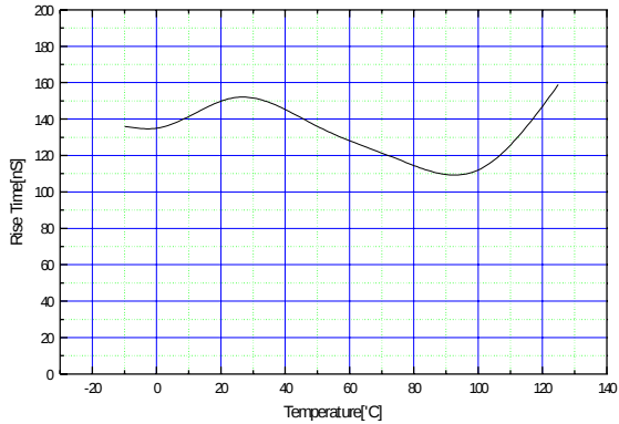
Figure 16. Rise Time vs Temperature
