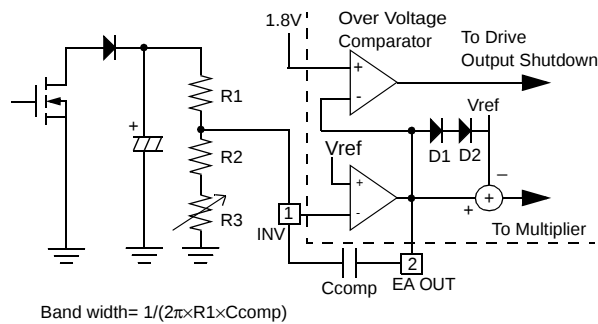
Figure 2.1 Error Amp and Over Voltage Comparator
