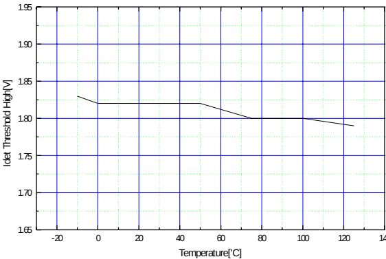
Figure 12. Idet Threshold High vs Temperature
