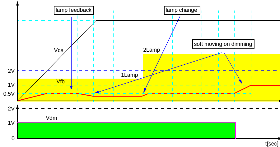
Figure 1. Operation Characteristics
