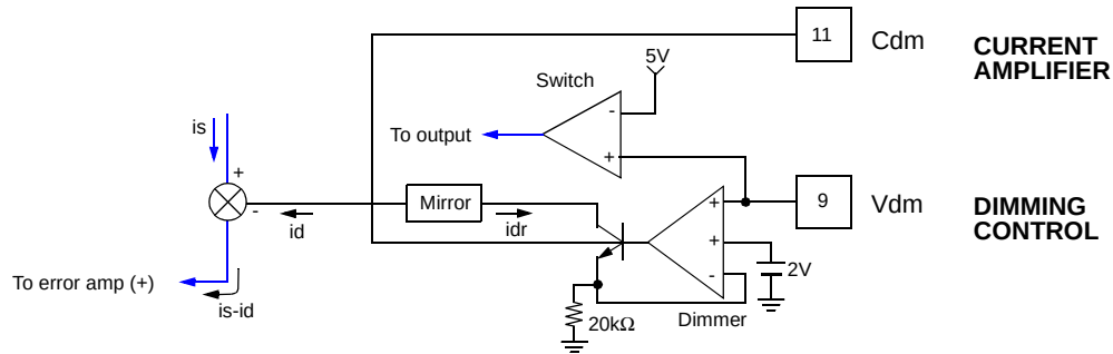
Figure 5. Dimming Control Stage
