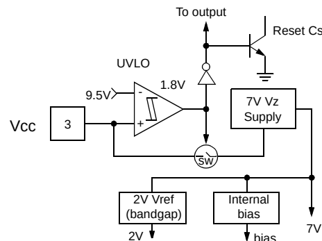
Figure 2. UVLO
