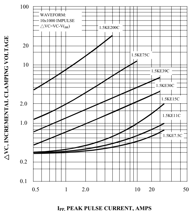
FIG. 10 - INCREMENTAL CLAMPING VOLTAGE CURVE BIDIRECTIONAL
