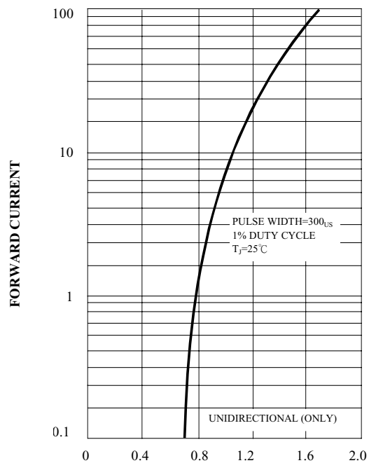
FIG. 11 - INSTANTANEOUS FORWARD VOLTAGE CHARACTERISTICS CURVE
