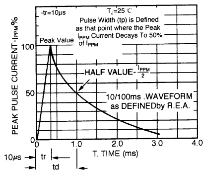
FIGURE 3 – PULSE WAVEFORM
