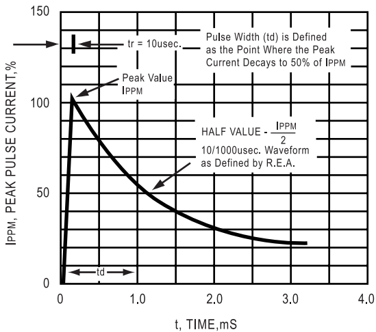
FIG. 3 - PULSE WAVEFORM
