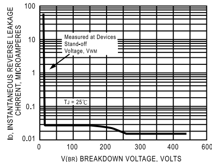
FIG. 7 - TYPICAL REVERSE LEAKAGE CHARACTERISTICS
