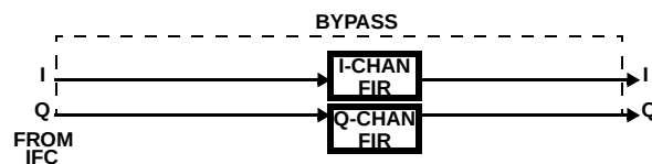
FIGURE 10. CORRECTION FILTER IN COMPLEX MODE
