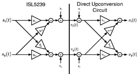
FIGURE 11. IMBALANCE CORRECTION
