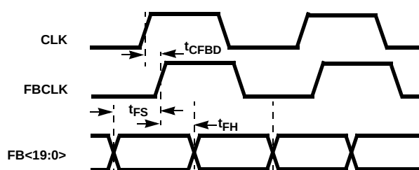
FIGURE 19. FEEDBACK TIMING
