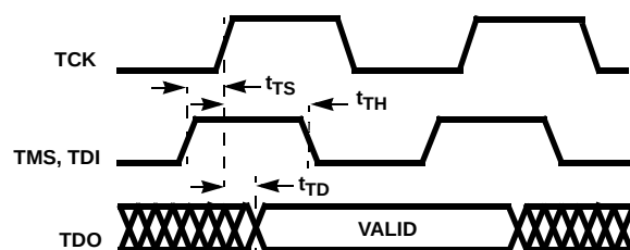
FIGURE 20. JTAG TIMING
