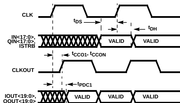
FIGURE 17. INPUT/OUTPUT TIMING
