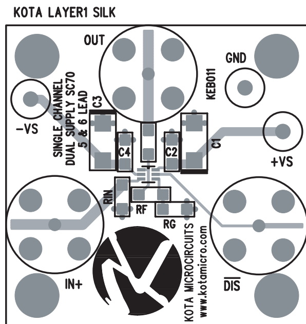
Figure 6c: KEB011 (top side)
