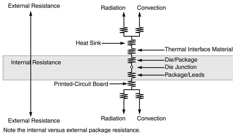
Figure 27. C4 Package with Heat Sink Mounted to a Printed-Circuit Board
