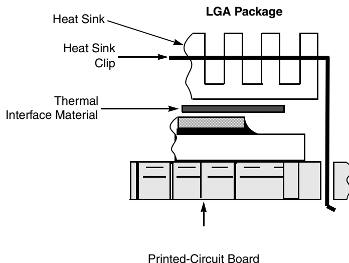
Figure 26. LGA Package Exploded Cross-Sectional View with Several Heat Sink Options
