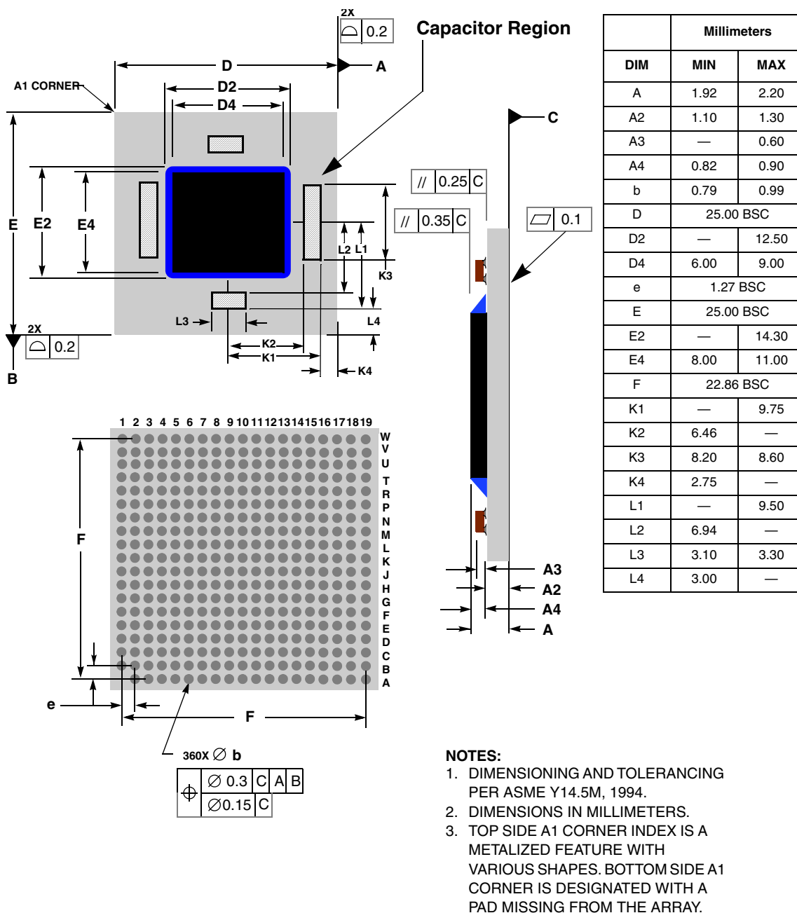
Figure 18. Mechanical Dimensions and Bottom Surface Nomenclature for the MPC7410, 360 HCTE_LGA Package
