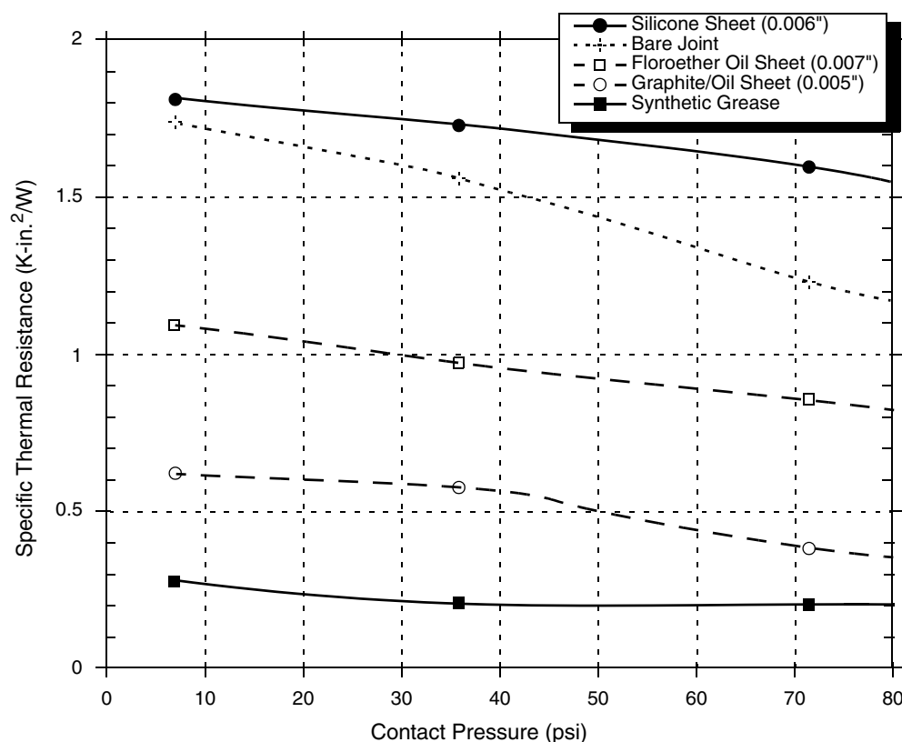
Figure 28. Thermal Performance of Select Thermal Interface Material
