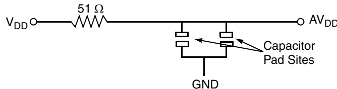
Figure 21. PLL Power Supply Filter Circuit No. 2
