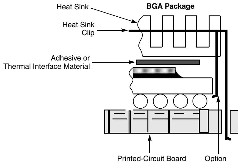
Figure 25. BGA Package Exploded Cross-Sectional View with Several Heat Sink Options
