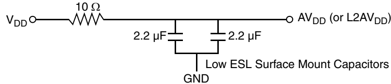
Figure 20. PLL Power Supply Filter Circuit No.1
