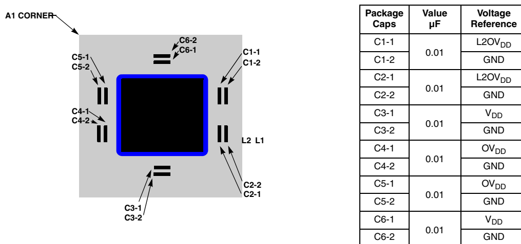
Figure 19. Substrate Bypass Capacitors for the MPC7410
