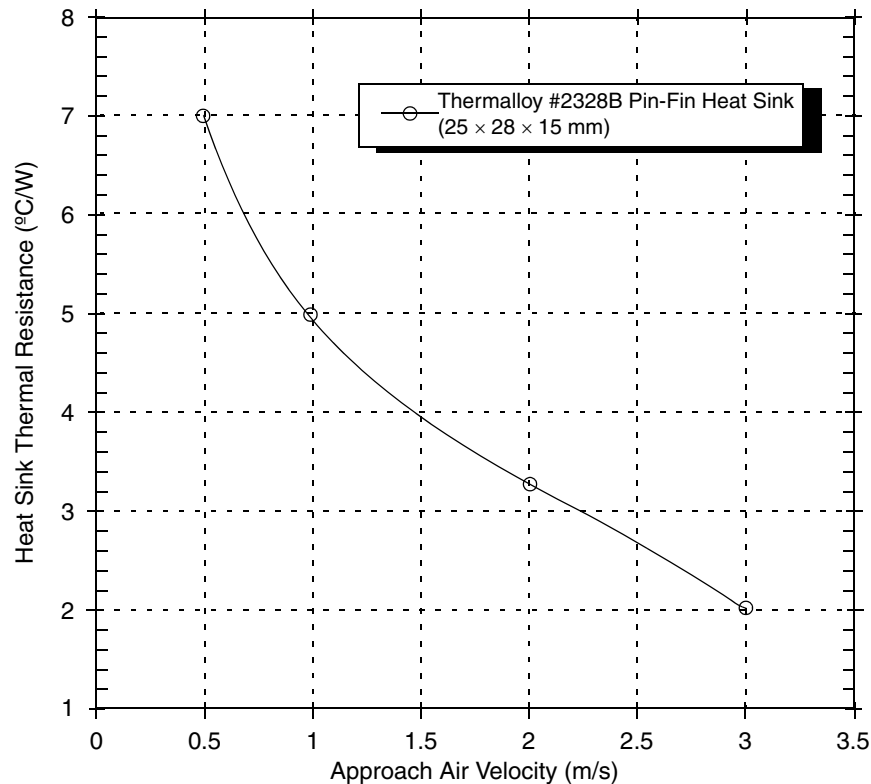
Figure 29. Thermalloy #2328B Heat Sink-to-Ambient Thermal Resistance Versus Airflow Velocity
