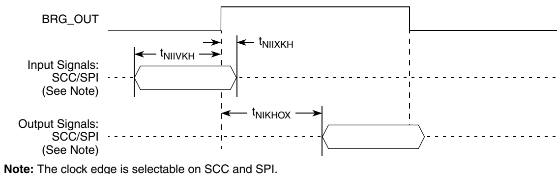
Figure 27. SCC/SPI AC Timing Internal Clock Diagram
