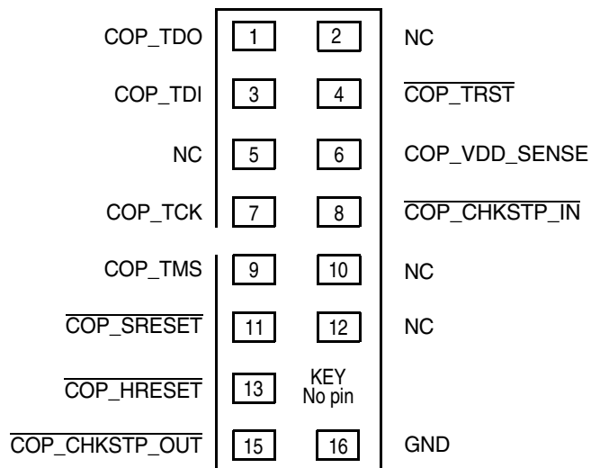
Figure 59. COP Connector Physical Pinout
