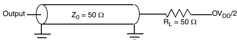
Figure 37. PCI/PCI-X AC Test Load
