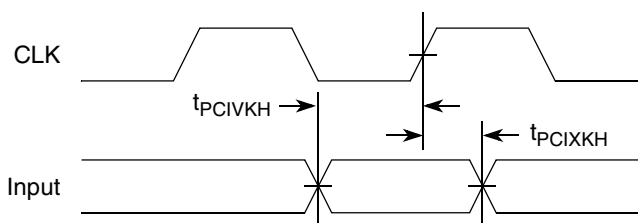
Figure 38. PCI-PCI-X Input AC Timing Measurement Conditions
