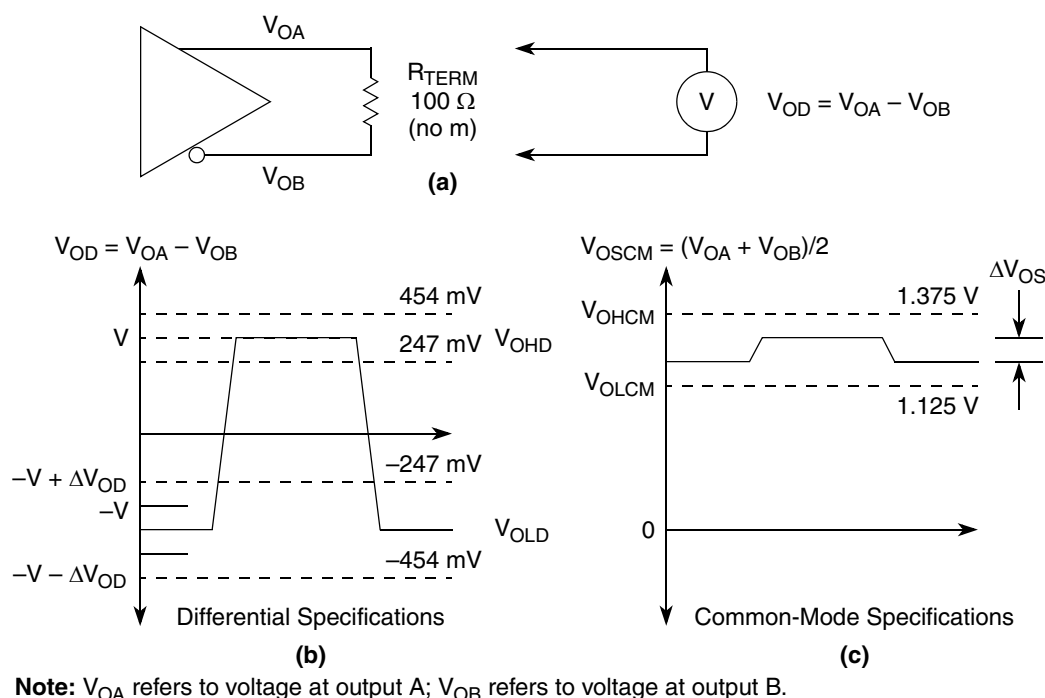
Figure 40. DC Driver Signal Levels
