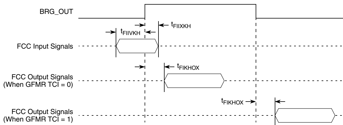
Figure 23. FCC Internal AC Timing Clock Diagram
