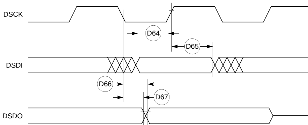
Figure 32. Debug Port Timings
