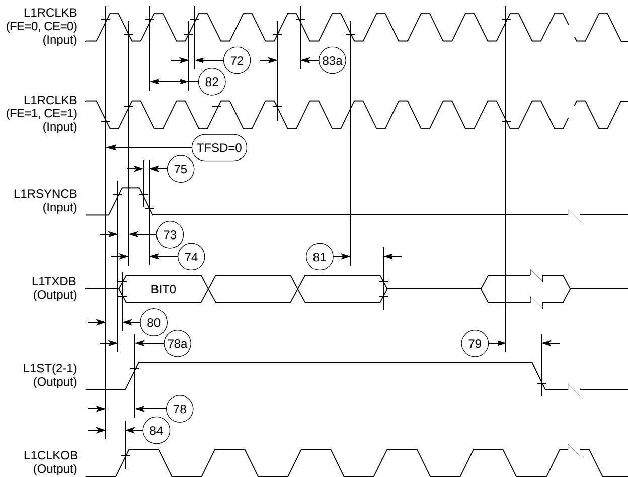
Figure 50. SI Transmit Timing with Double Speed Clocking (DSC = 1)
