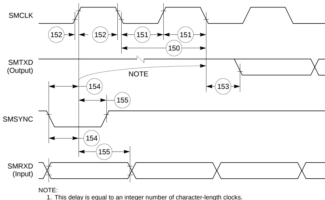
Figure 58. SMC Transparent Timing Diagram
