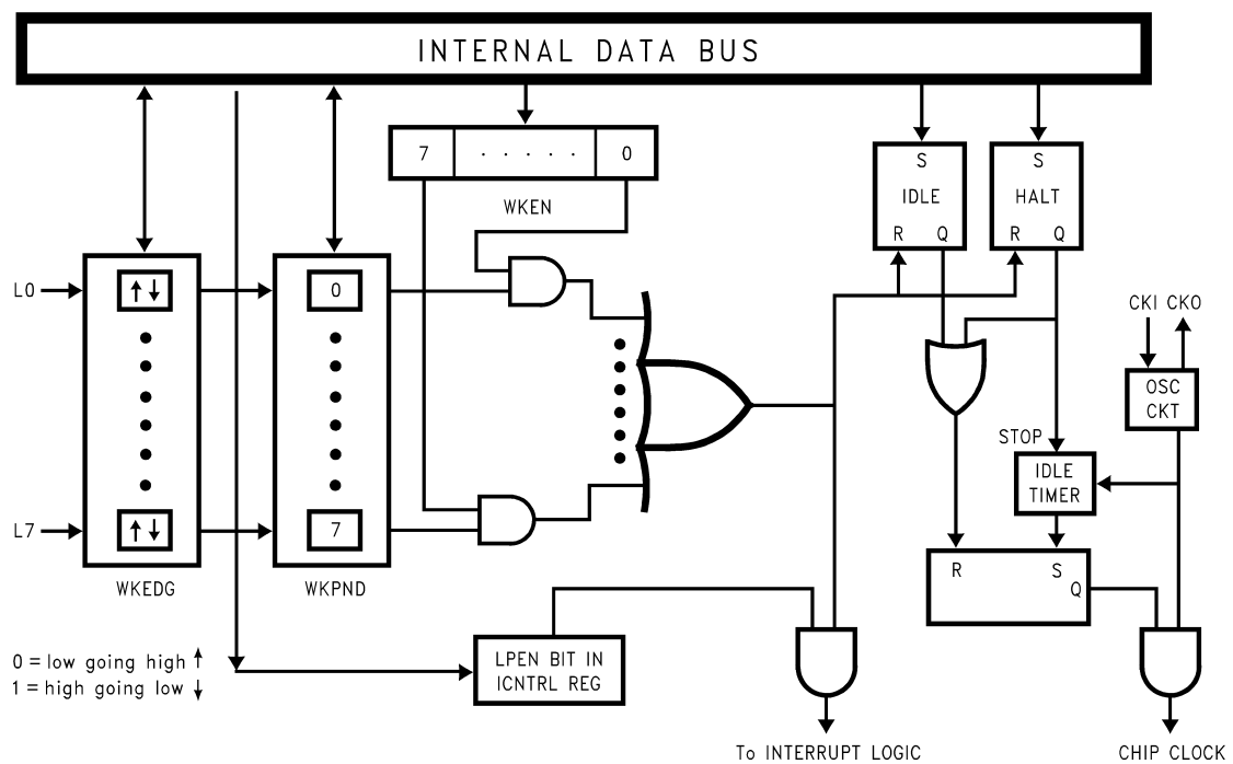
FIGURE 21. Multi-Input Wake-Up Logic
