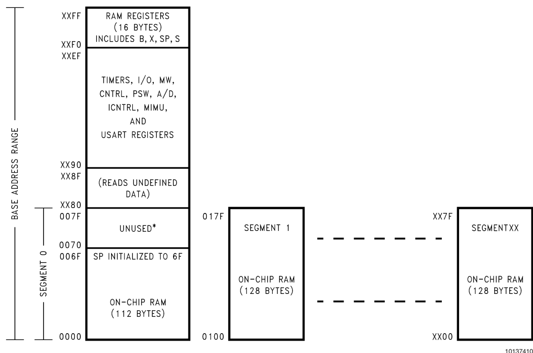
FIGURE 7. RAM Organization
