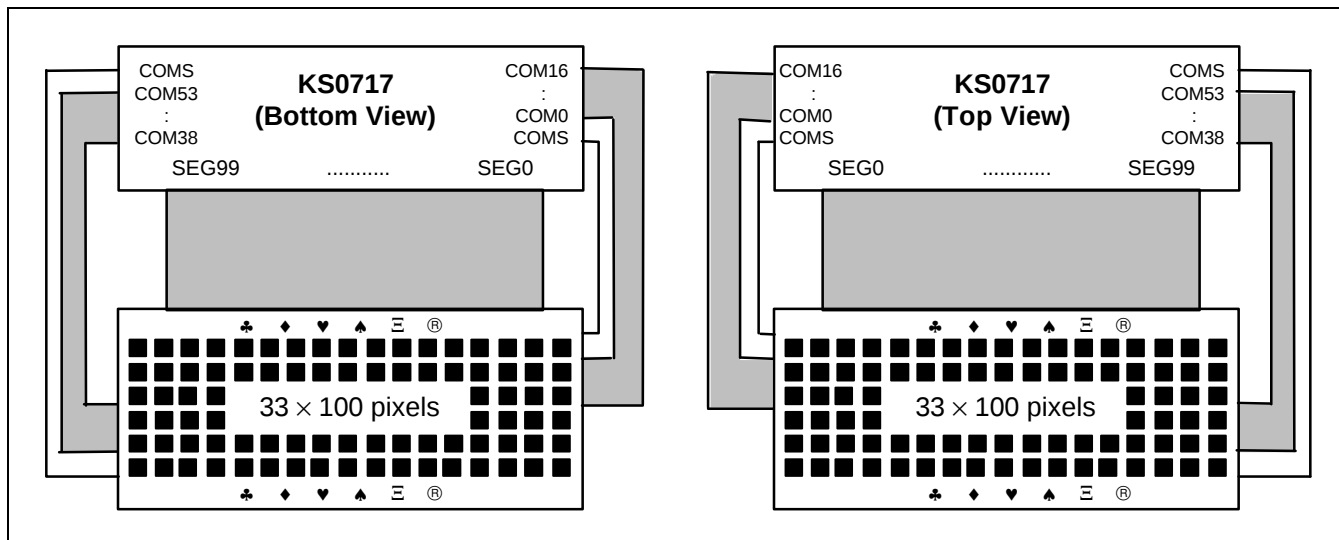
Figure 46. SHL = 0, ADC = 1
