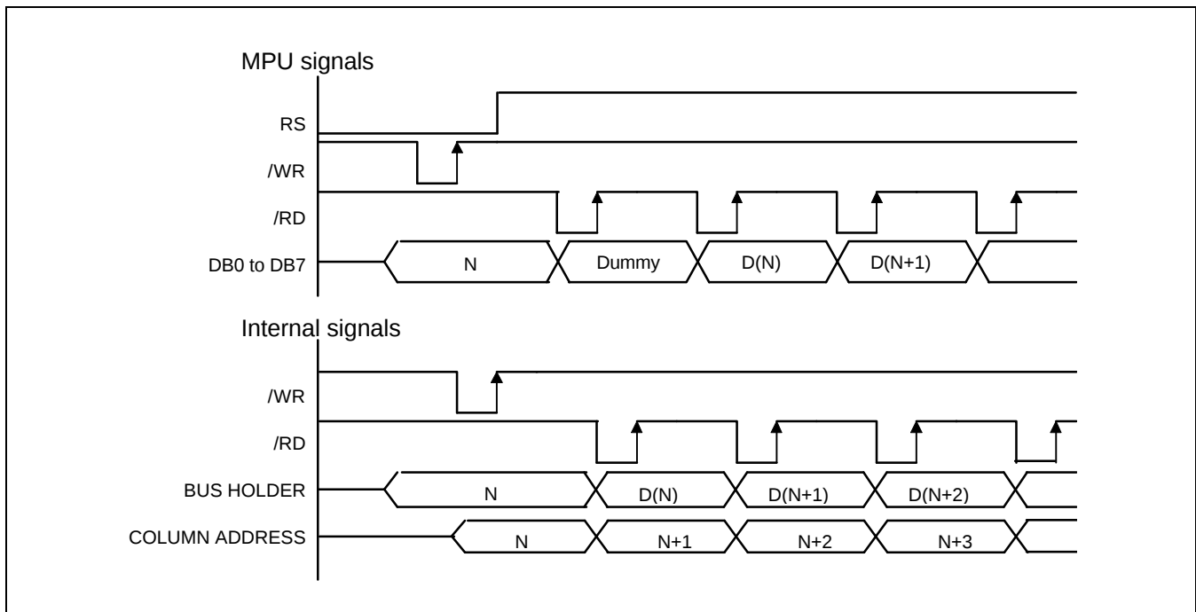
Figure 5. Read Timing
