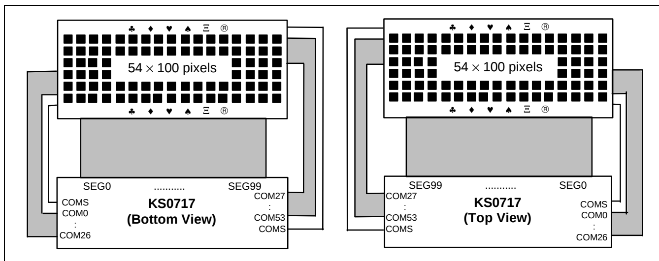
Figure 44. SHL = 1, ADC = 0
