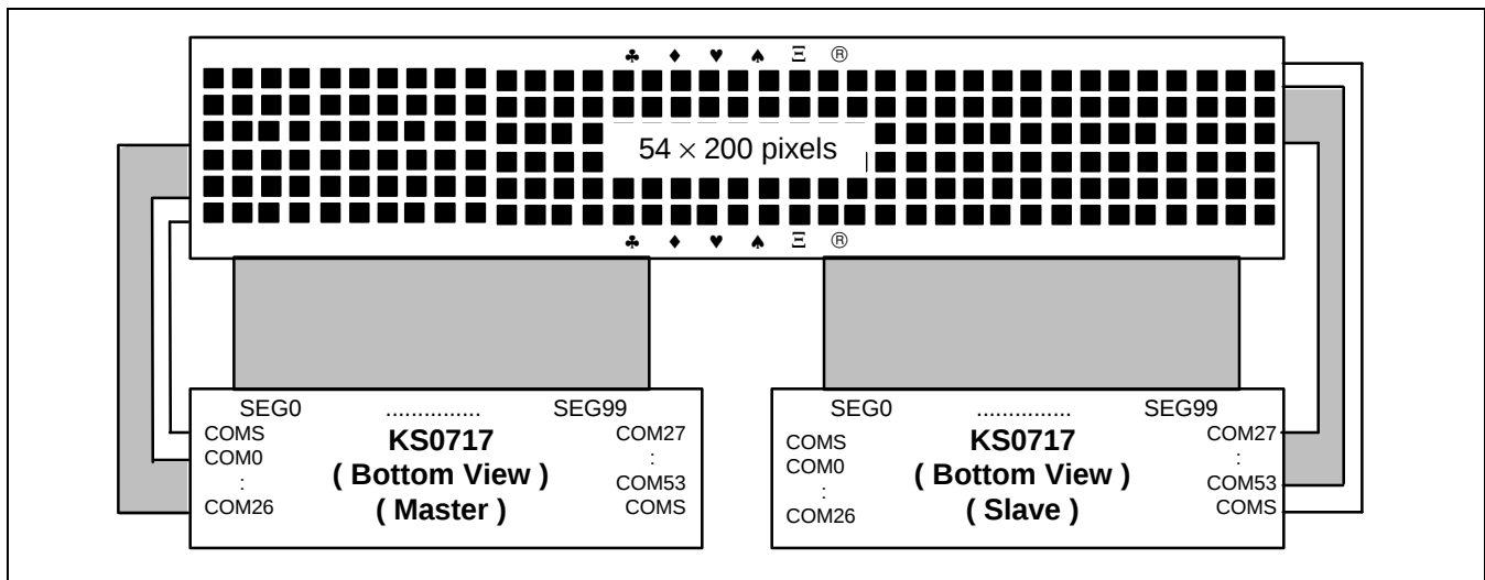
Figure 51. SHL = 1, ADC = 0
