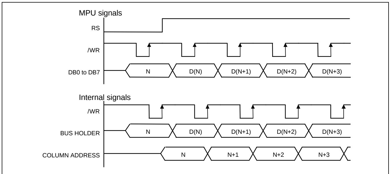
Figure 4. Write Timing
