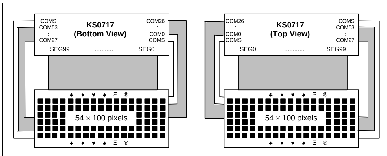
Figure 42. SHL = 0, ADC = 1
