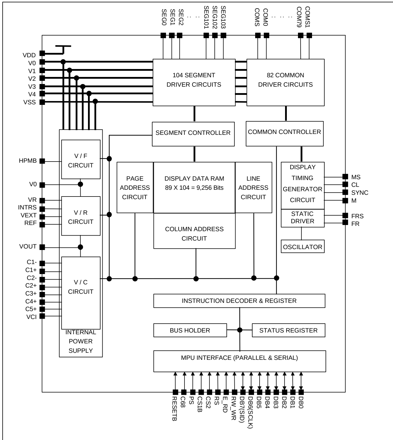
Figure 1. Block Diagram
