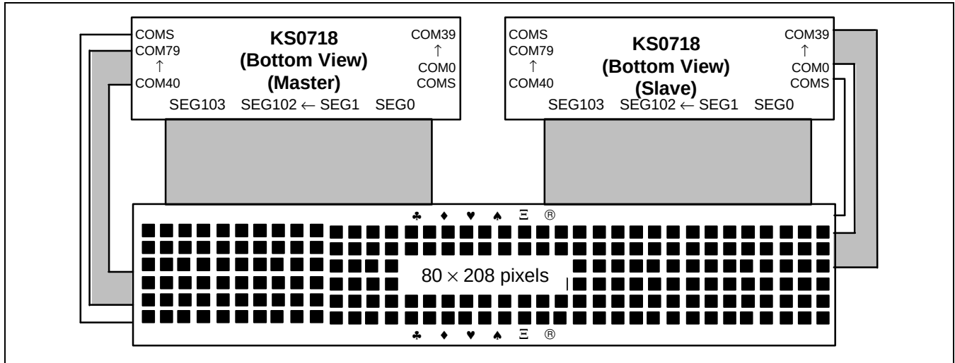
Figure 51. SHL = 0, ADC = 1
