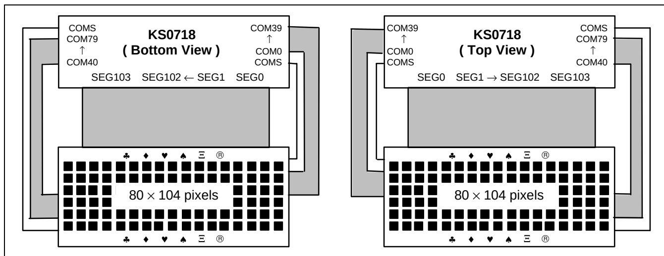
Figure 47. SHL = 0, ADC = 1
