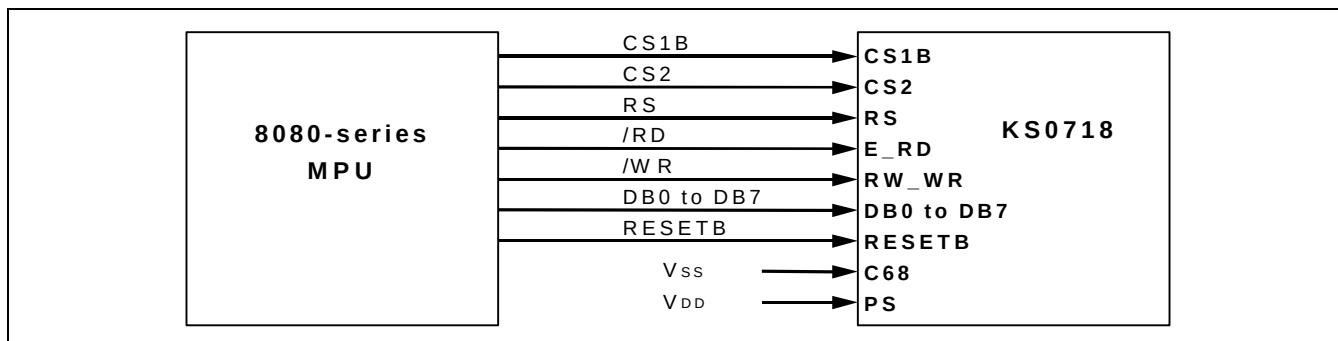
Figure 45. In Case of Interfacing with 8080-series (PS = "H", C68 = "L")
