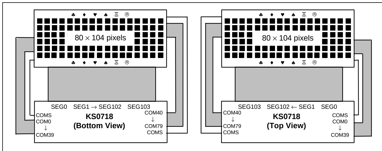
Figure 49. SHL = 1, ADC = 0
