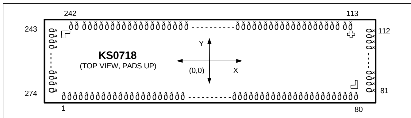
Figure 2. KS0718 Chip Configuration
