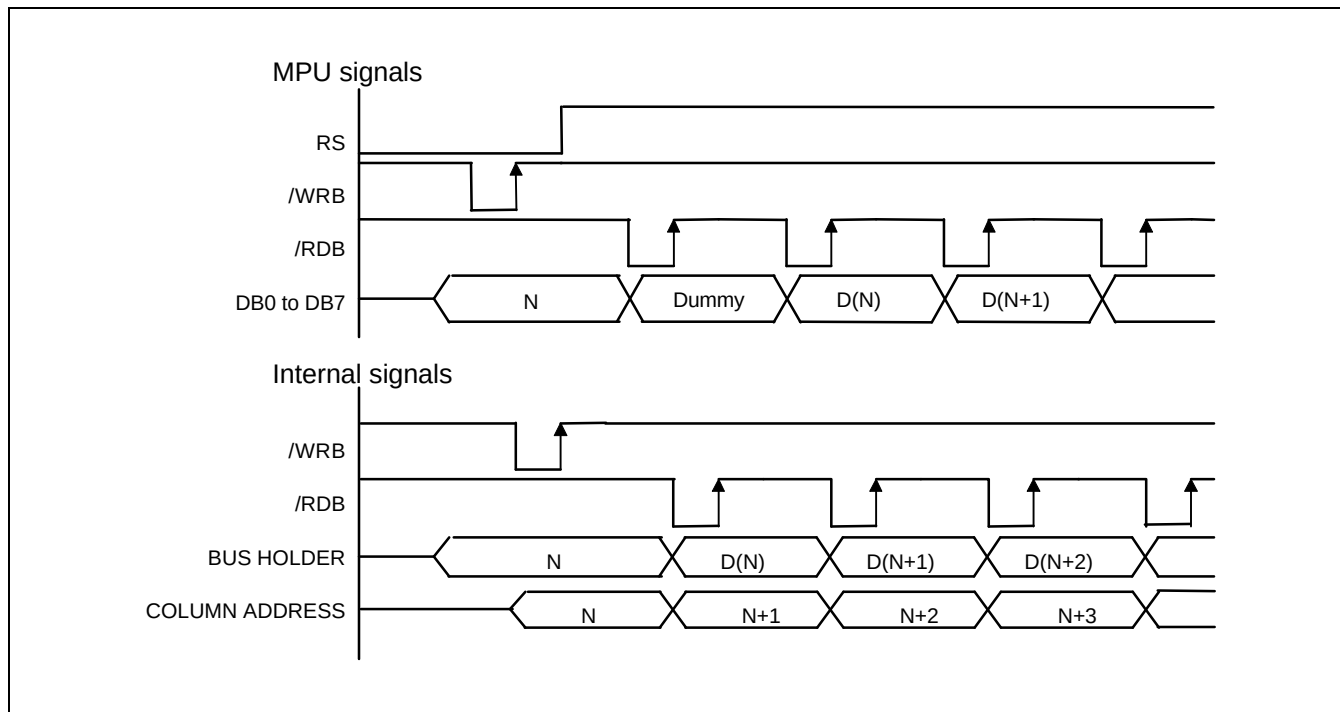
Figure 5. Read Timing
