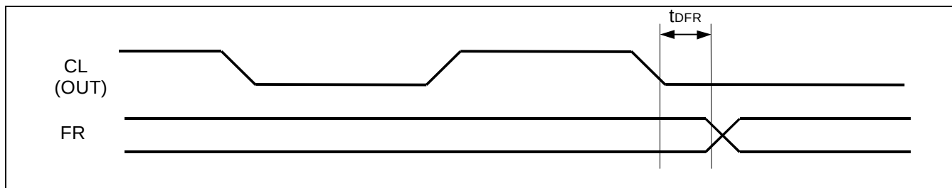
Figure 34. Display Control Output Timing
