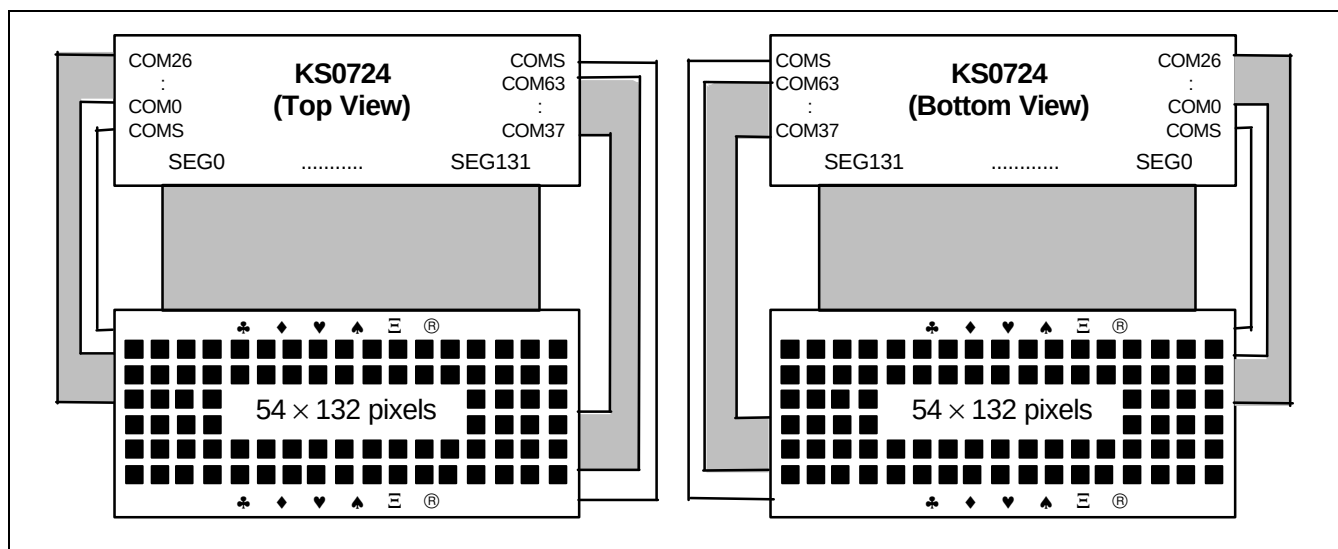
Figure 44. SHL = 0, ADC = 0
