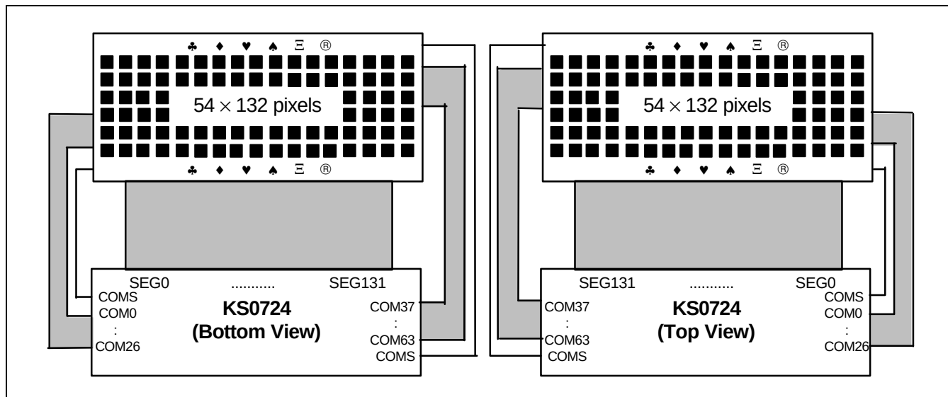
Figure 42. SHL = 1, ADC = 0
