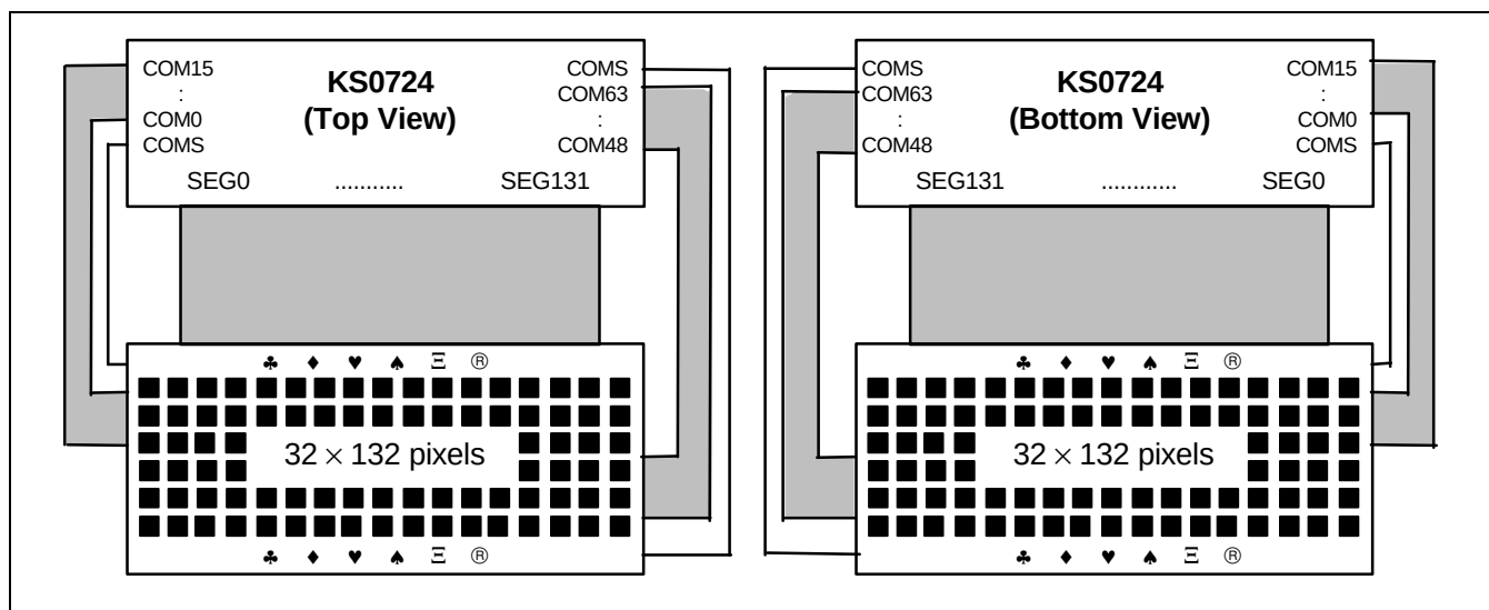
Figure 52. SHL = 0, ADC = 0
