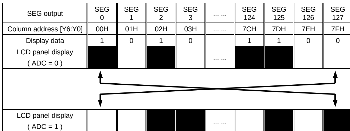
Figure 8. The Relationship between the Column Address and the Segment Outputs
