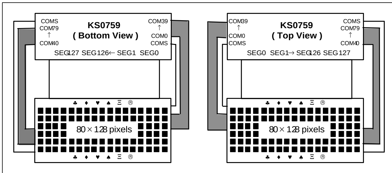
Figure 49. SHL = 0, ADC = 1
