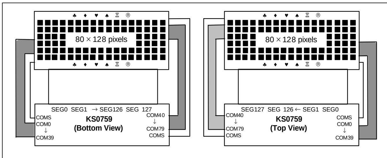
Figure 51. SHL = 1, ADC = 0
