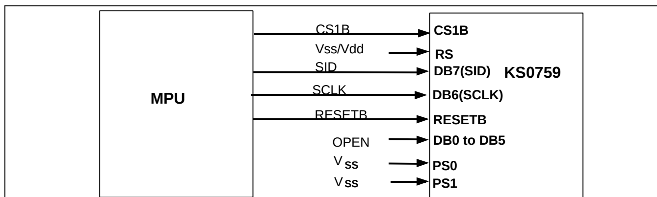
Figure 48. Serial Interface
