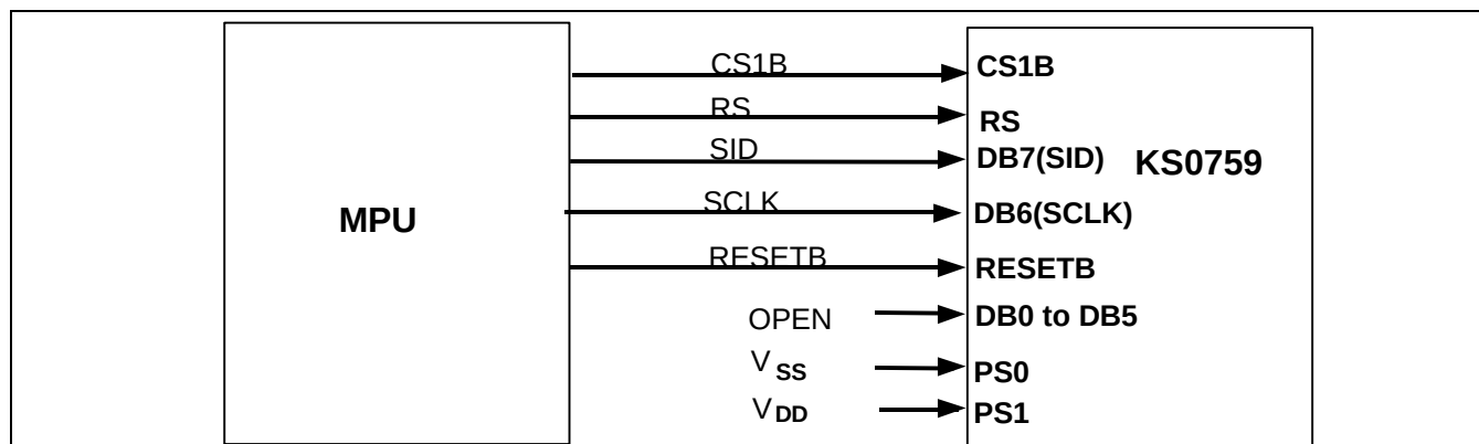
Figure 47. Serial Interface
