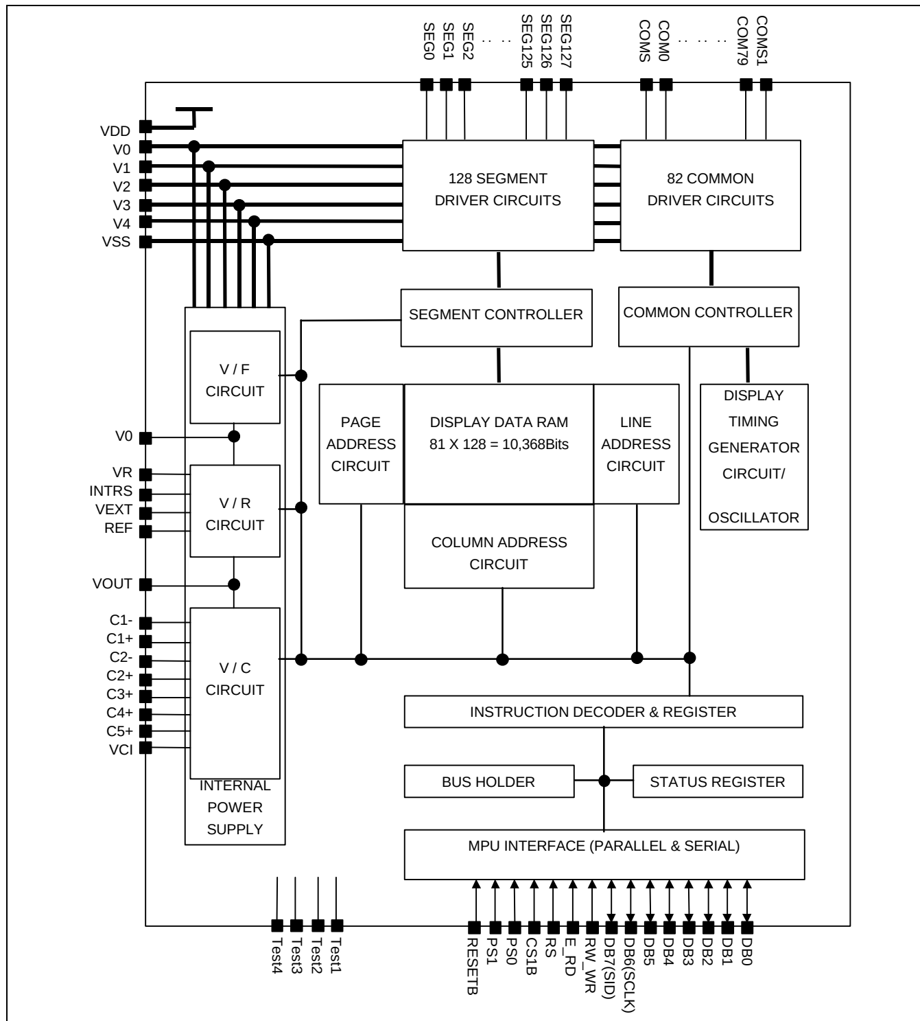
Figure 1. Block Diagram
