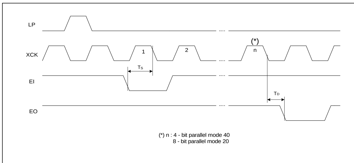
Figure 3-2. Timing Characteristics of Segment Mode
