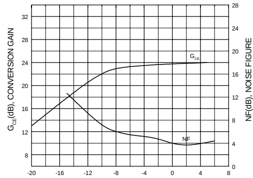
Figure 4. G_{CE} , NF-
