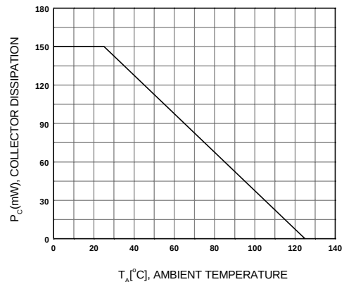
Figure 6. P_C - T_A
