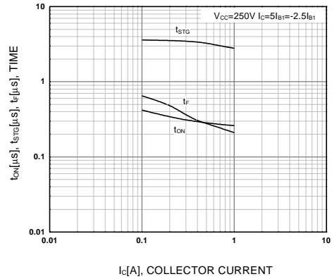
Figure 4. Switching Time
