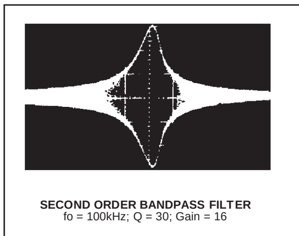
OUTPUT A
