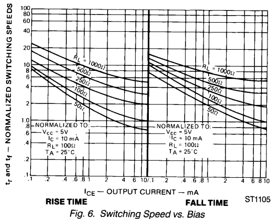
Fig. 6. Switching Speed vs. Bias ST1105
