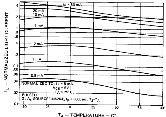
Fig. 4. Light Current vs. Temperature ST1106
